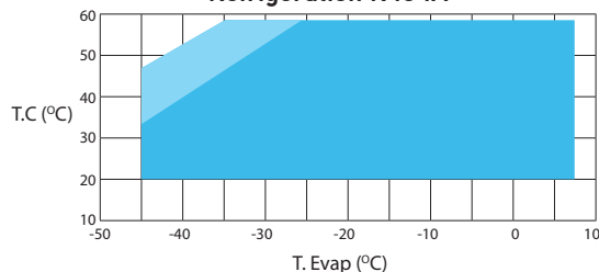
Refrigeration R404A
