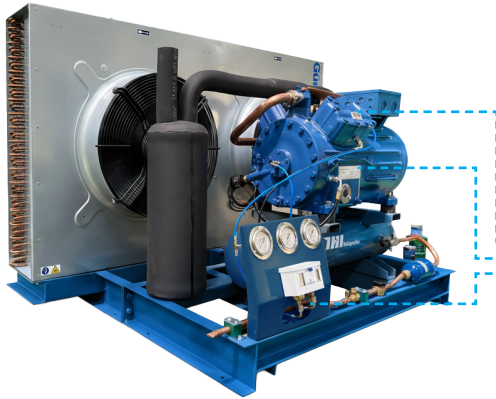
SINGLE STAGE WITH PANEL CONTROL
