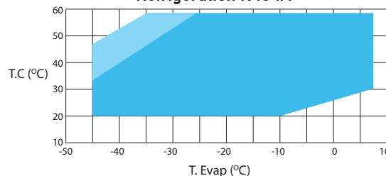
Refrigeration R404A
